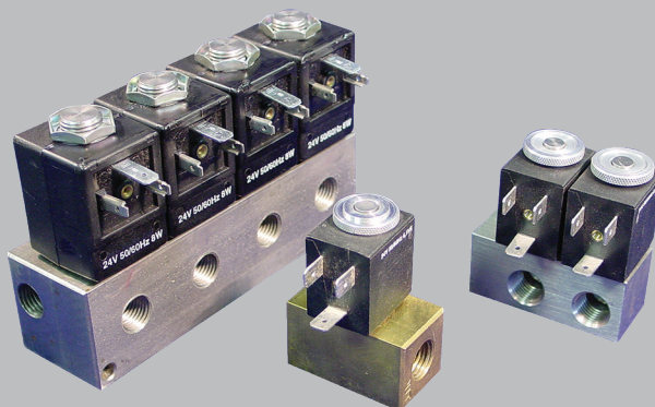
SPACESAVER MANIFOLDS S30, S31, S40, C4, C9 SERIES STAINLESS STEEL | BRASS | ALUMINUM | POLYMERS
