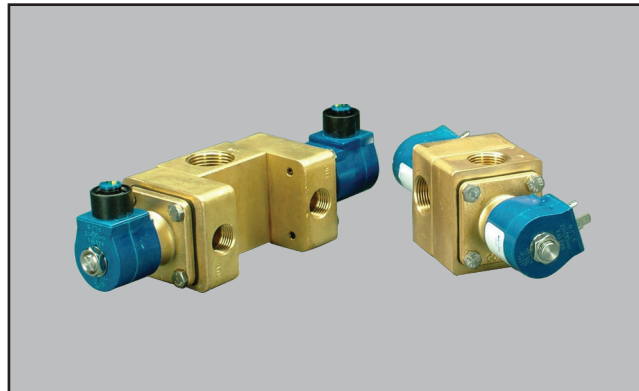
3-WAY HIGH FLOW | M20, M21 SERIES 3/8", 1/2", 3/4" NPT STAINLESS STEEL | BRASS | NORYL
